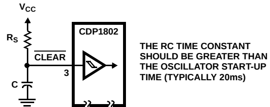
FIGURE 24. RESET DIAGRAM
