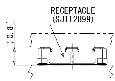
MATED CONDITION (REF.) 嵌合状態図 (参考)
