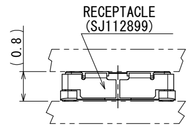
MATED CONDITION (REF.) 嵌合状態図 (参考)
