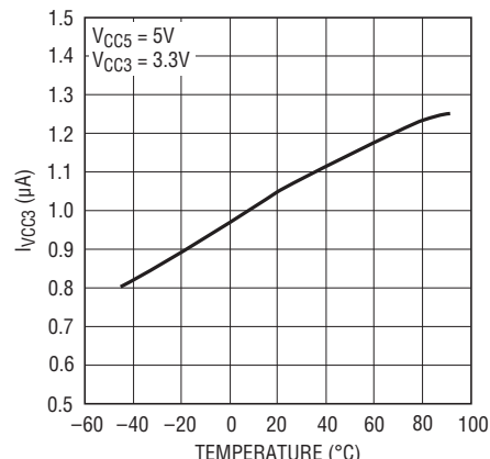
I_{VCC3} vs Temperature (LTC1726-5)
