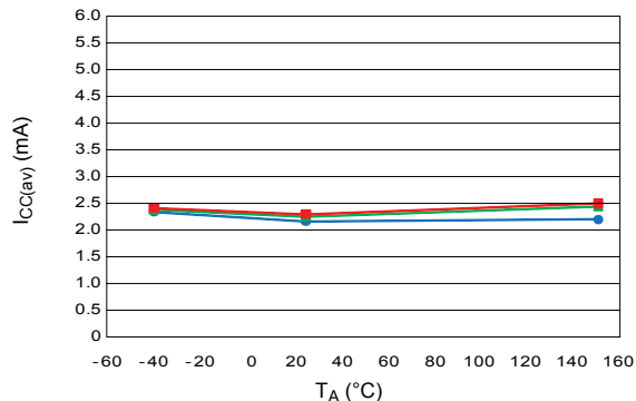
Average Supply Current (Off) versus Ambient Temperature
