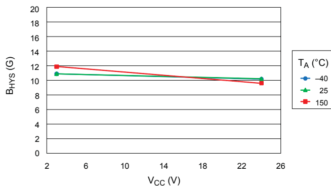
Average Switchpoint Hysteresis versus Supply Voltage
