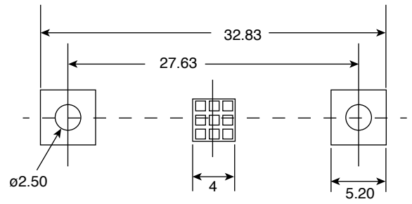
PBC Mounting Layout
