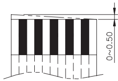
Tolerance of Cutting Tilt
