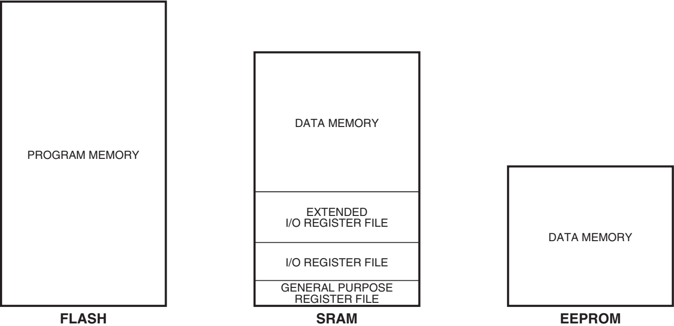
Figure 5-1. Memory Overview.
