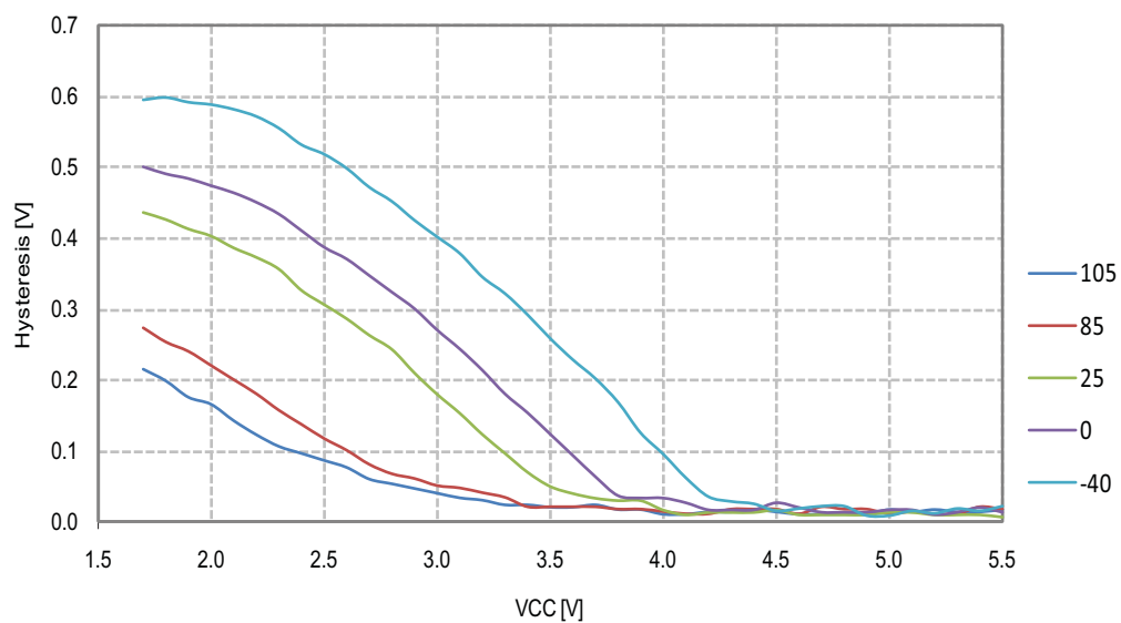
Figure 26-48.Reset Input Hysteresis vs. V_{CC}
