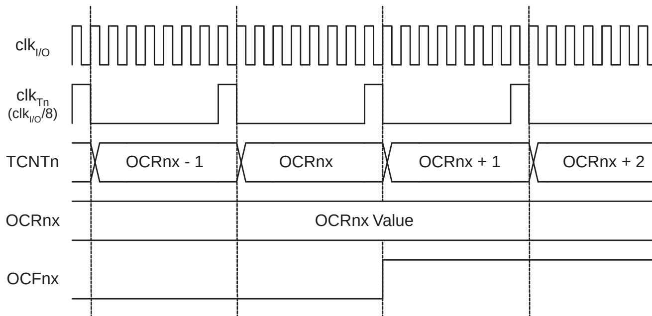
Figure 12-11. Timer/Counter Timing Diagram, Setting of OCFnx, with Prescaler ( f_{clk_{I/O}}/8 )
