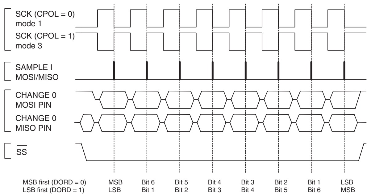
Figure 17-4. SPI Transfer Format with CPHA = 1
