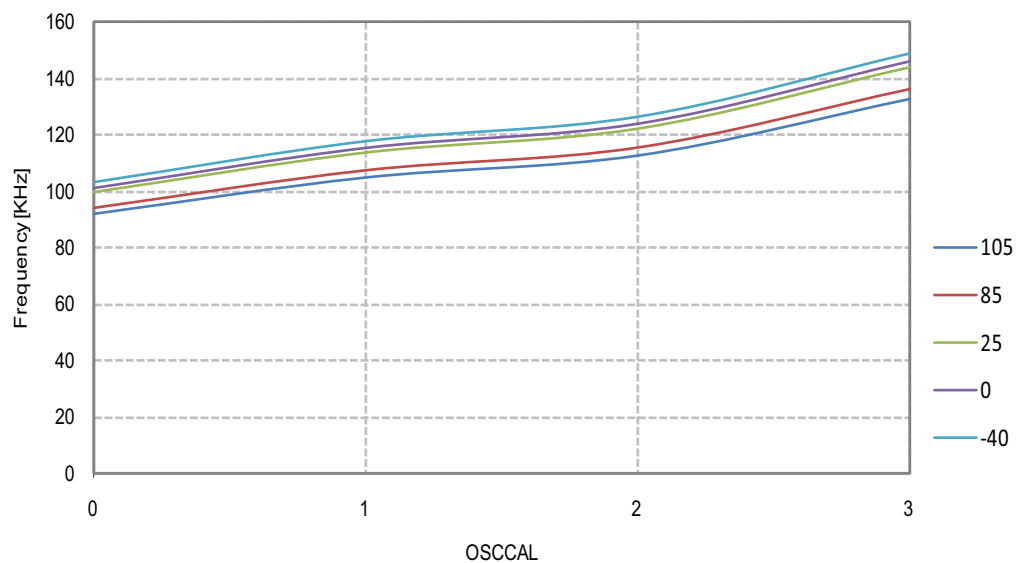
Figure 26-178. ULP 128kHz Calibrated Oscillator Frequency vs. OSCAL1 Value
