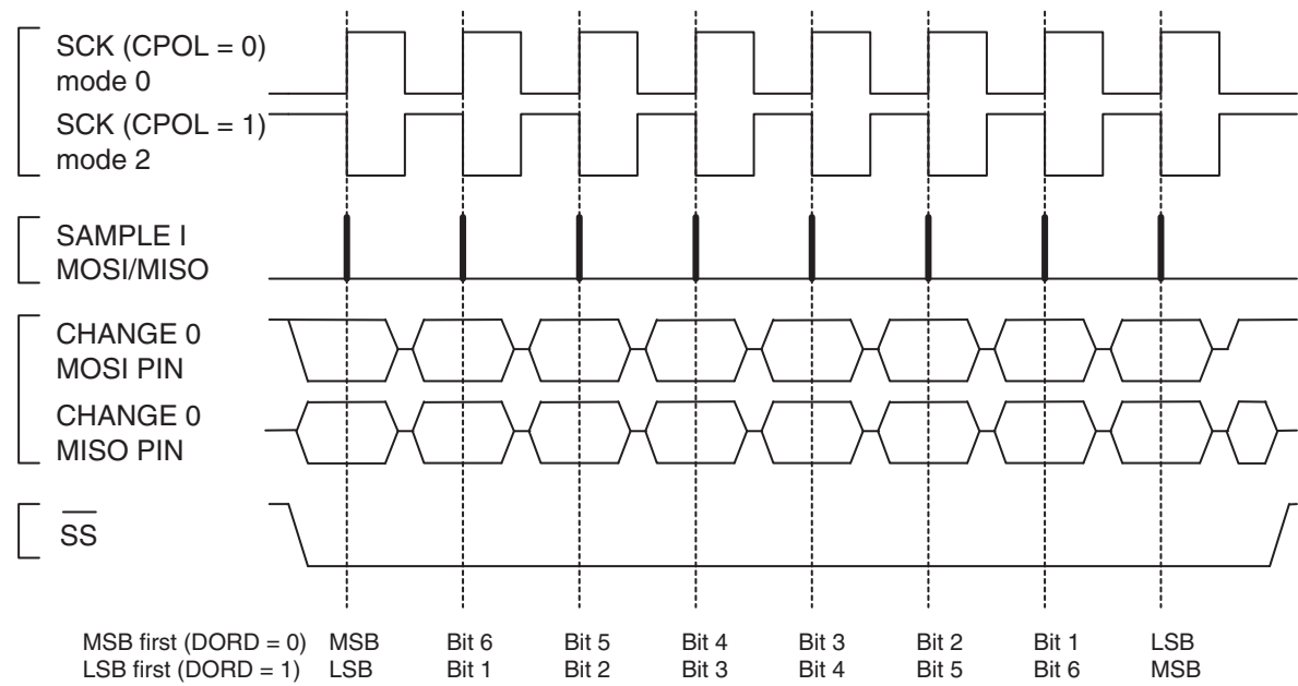
Figure 17-3. SPI Transfer Format with CPHA = 0
