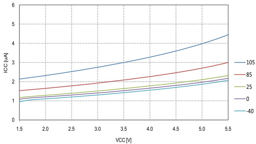
Figure 26-112.Power-down Supply Current vs. V CC , Watchdog Timer Enabled
