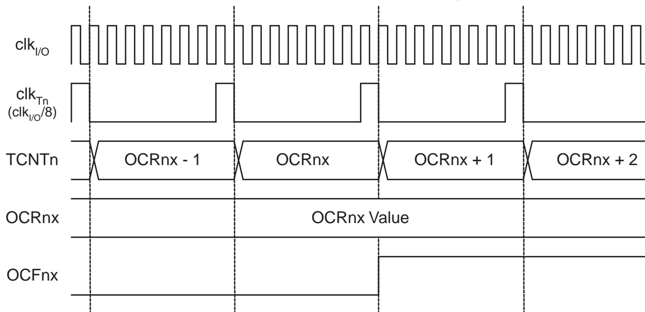
Figure 12-11. Timer/Counter Timing Diagram, Setting of OCFnx, with Prescaler ( f_{\text{clk\_I/O}}/8 )
