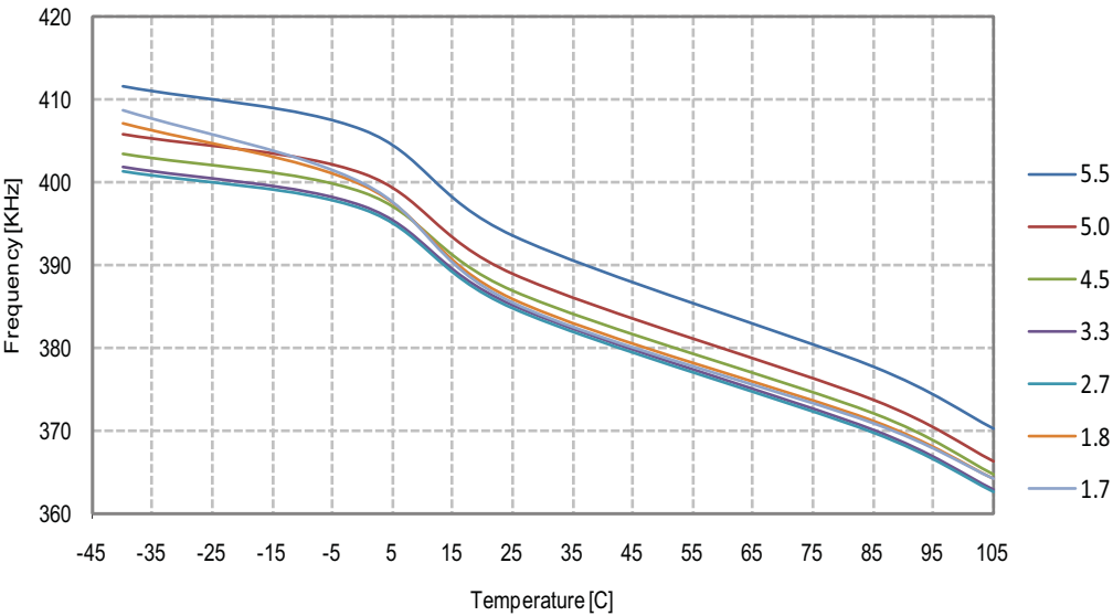
Figure 26-183. ULP 512kHz Oscillator, Frequency vs. Operating Temperature
