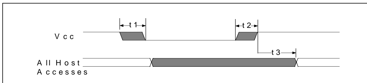
FIGURE 27-1: POWER-UP TIMING
