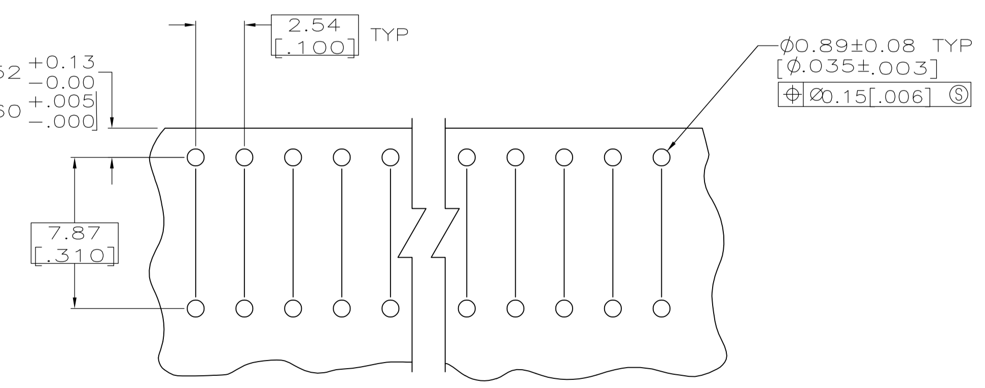
RECOMMENDED PC BOARD HOLE LAYOUT
