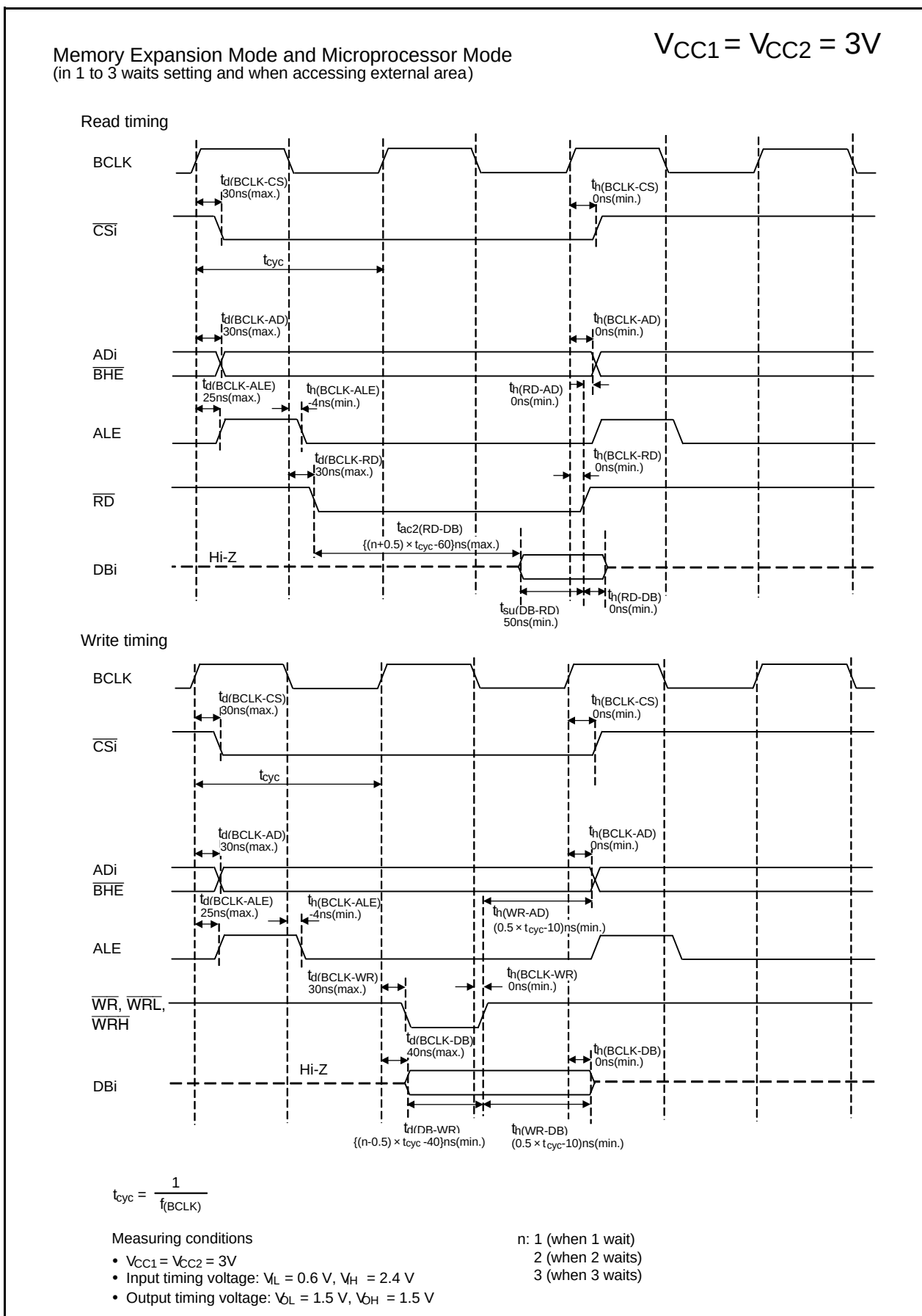
Figure 5.29 Timing Diagram
