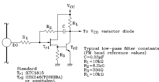
Typical Active Low-Pass Filter Circuit
