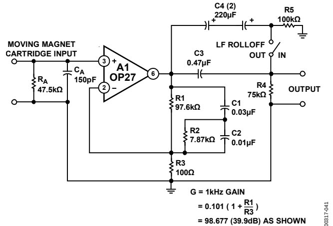
Figure 41. Phono Preamplifier Circuit
