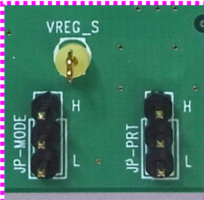
Figure 5. Appearance of JP-MODE, JP-PRT
