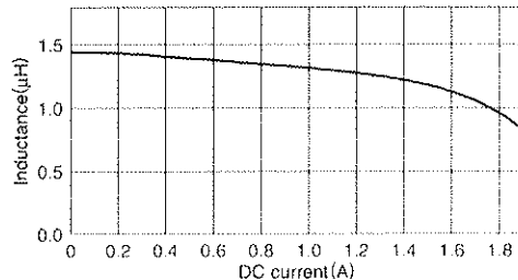
VLS252010T-1R5N
