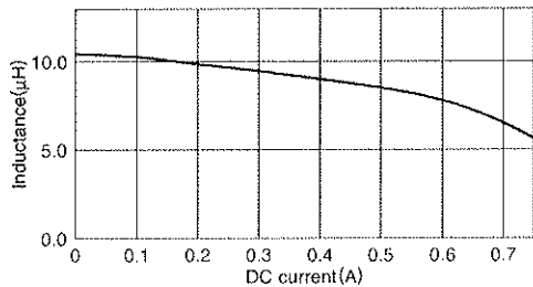
VLS252010T-100M
