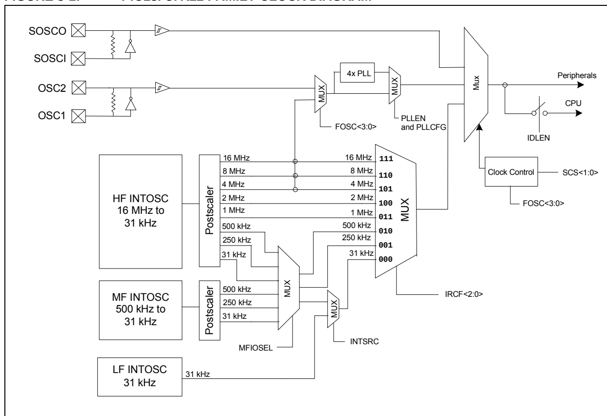
FIGURE 3-1: PIC18F87K22 FAMILY CLOCK DIAGRAM
