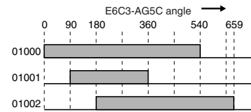
Output Timing
