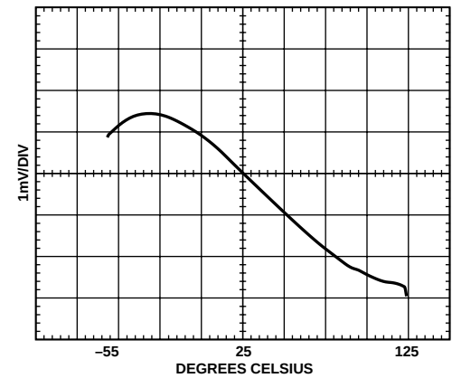
Figure 13. Reference Drift
