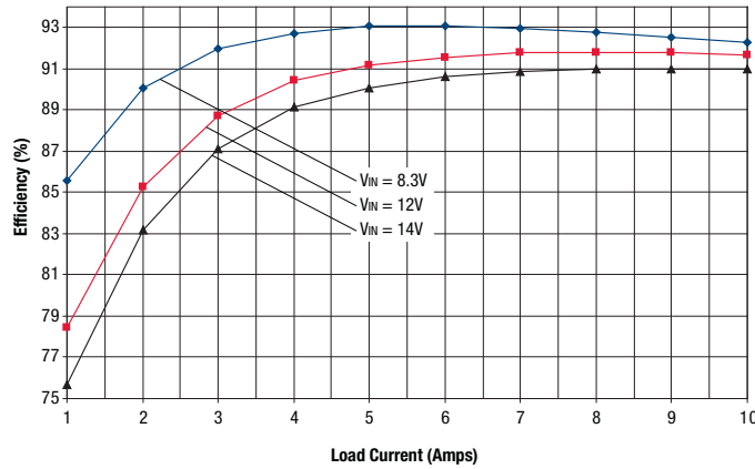
OKX2-T/10-D12 Efficiency vs. Line Voltage and Load Current @ +25°C (V OUT = 2.5V)
