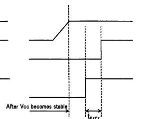
Fig.-3(b) SCL='L' and SDA='L'
