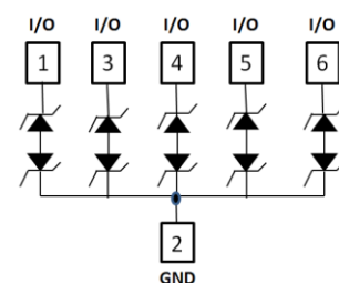
Device Schematic
