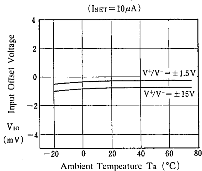
Input Offset Voltage vs. Ambient Temperature
