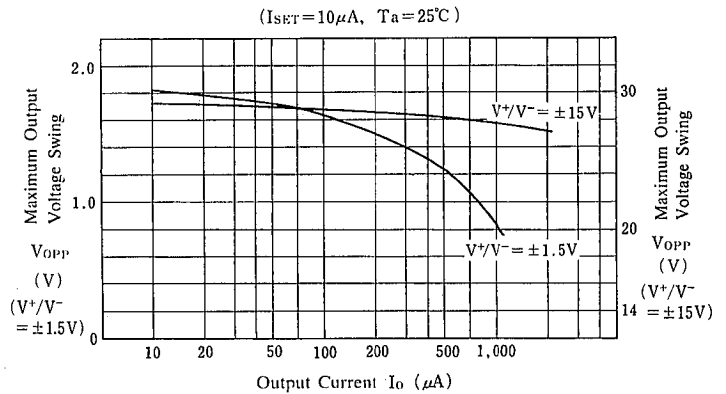
Maximum Output Voltage Swing vs. Output Current
