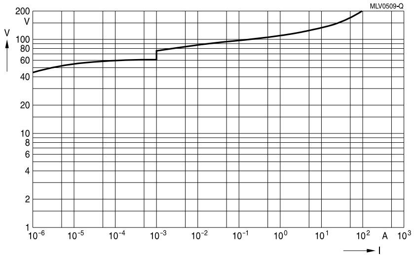
CT1206K40G
