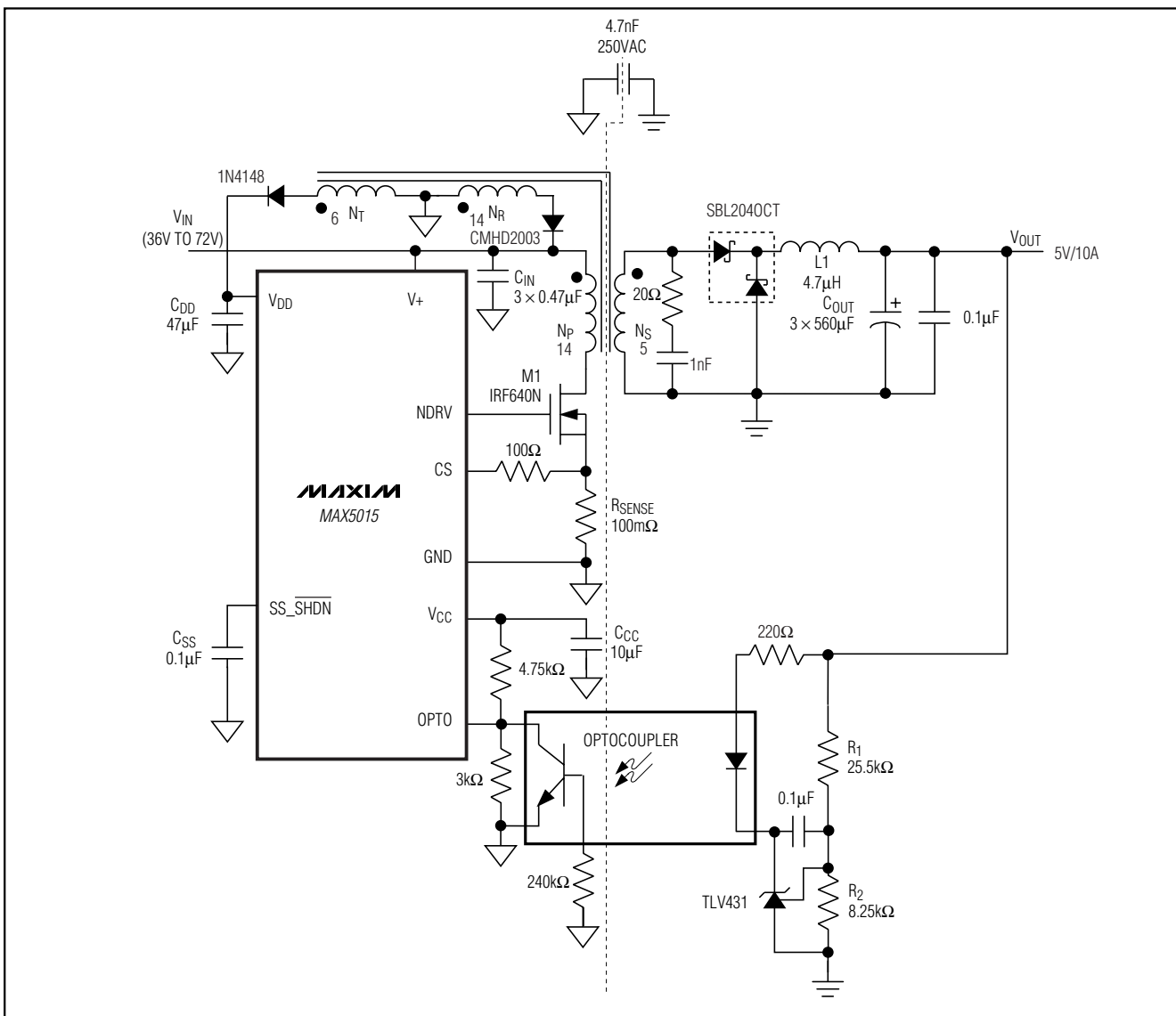
Figure 2. Forward Converter
