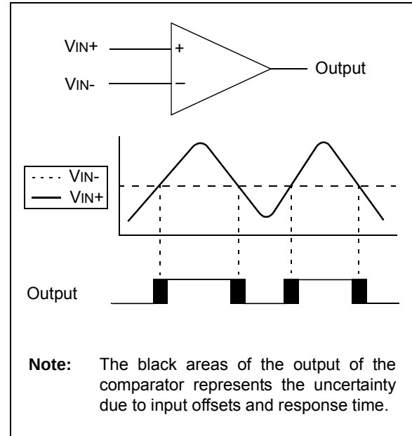
FIGURE 19-1: SINGLE COMPARATOR
