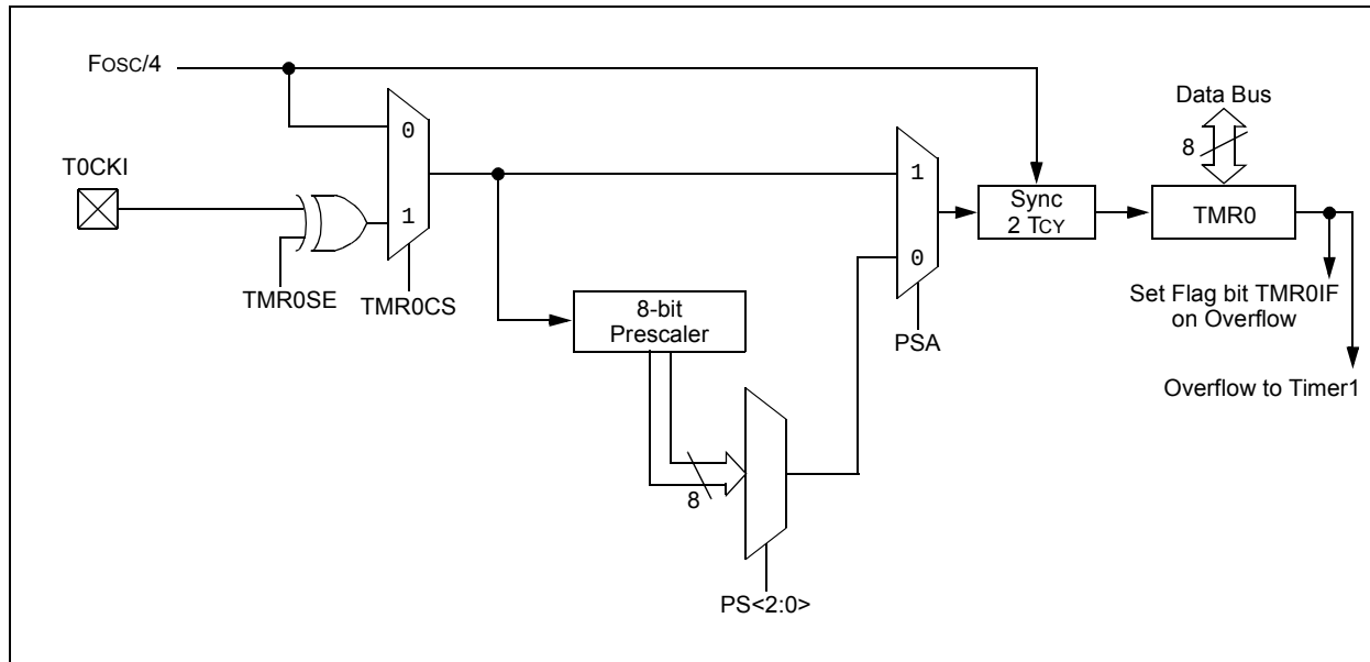
FIGURE 20-2: BLOCK DIAGRAM OF THE TMR0
