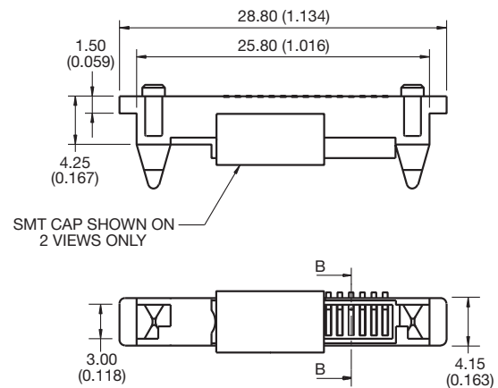
SMT Plug without Coax
