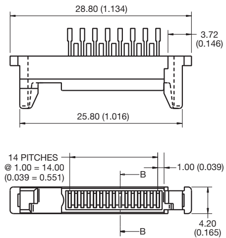
Plug Wire without Coax
