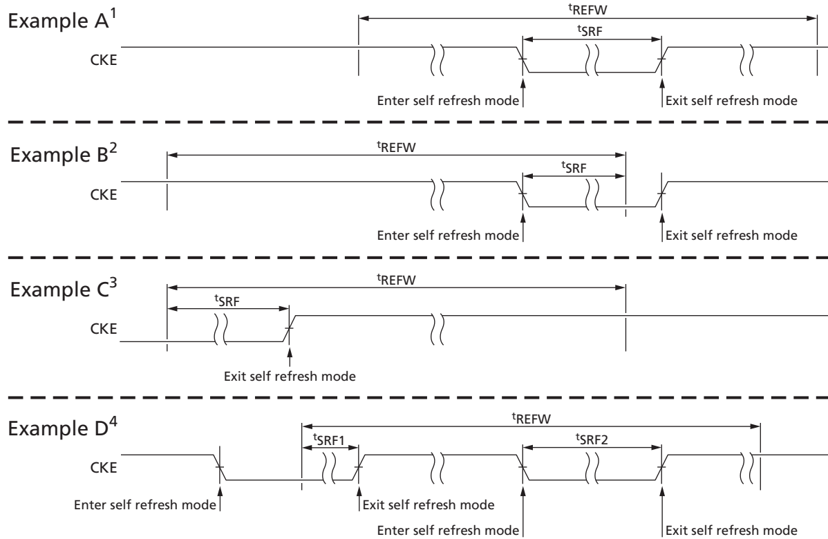
Figure 46: t_{SRF} Definition
