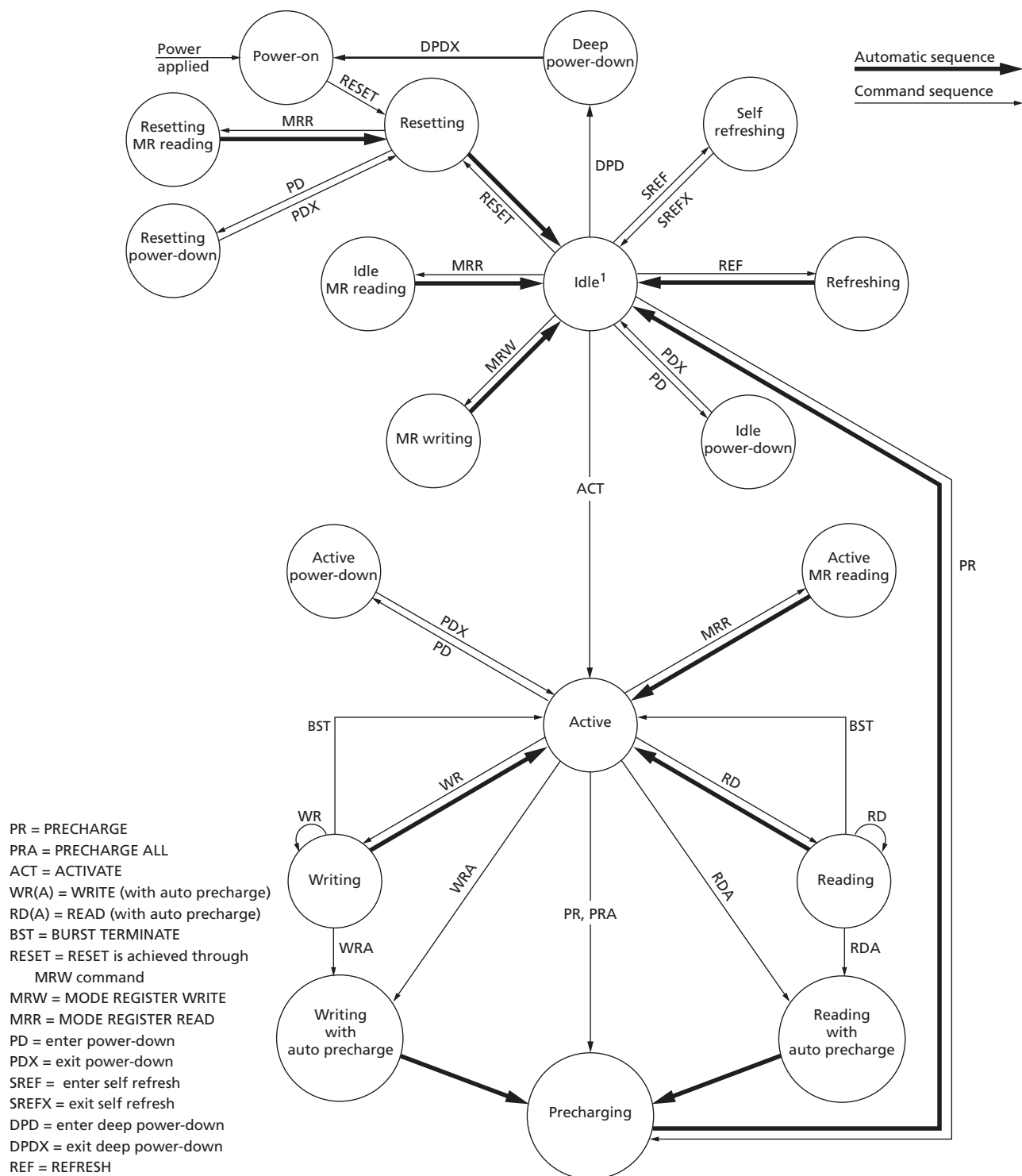
Figure 70: Simplified Bus Interface State Diagram
