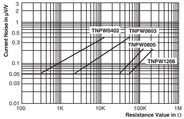
Current Noise
