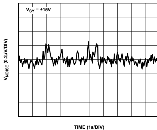
Figure 22. 0.1 Hz to 10 Hz Input Voltage Noise
