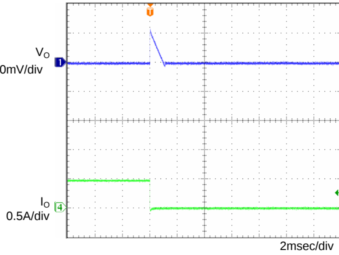
Fig.6 Transient Response (0.5→0A) Co=1μF, Ta=-40°C
