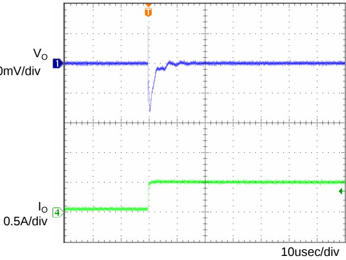
Fig.4 Transient Response (0→0.5A) Co=1μF, Ta=25°C
