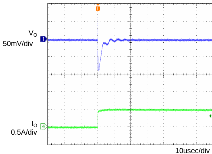
Fig.5 Transient Response (0→0.5A) Co=1 \mu F, T_a = 105^\circ\text{C}
