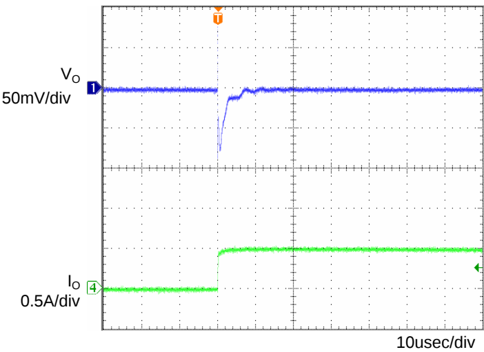
Fig.3 Transient Response (0→0.5A) Co=1 \mu F, T_a = -40^\circ\text{C}
