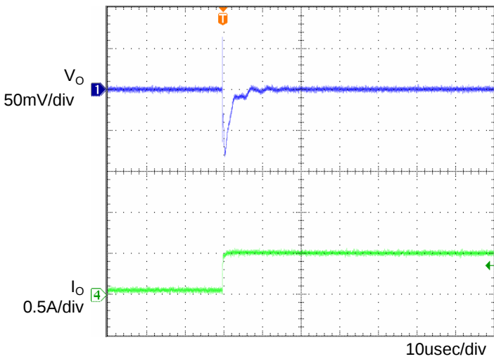
Fig.4 Transient Response (0→0.5A) Co=1 \mu F, T_a = 25^\circ\text{C}
