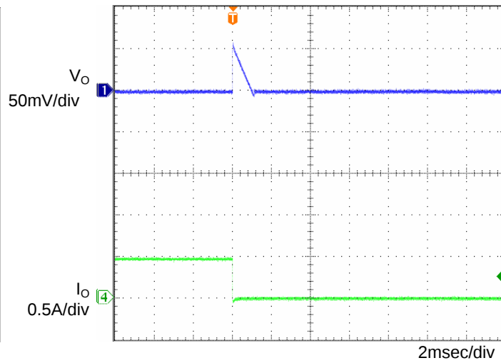
Fig.6 Transient Response (0.5→0A) Co=1 \mu F, T_a = -40^\circ\text{C}
