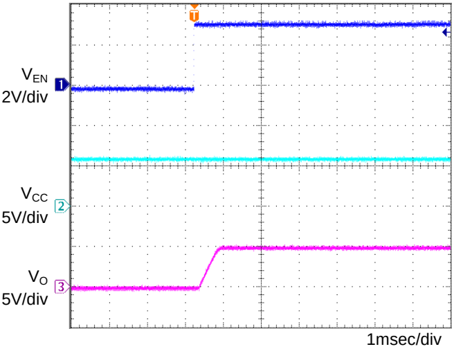
Fig.15 Input sequence 2 \text{Co}=1\mu\text{F} , T_a=-40^{\circ}\text{C}
