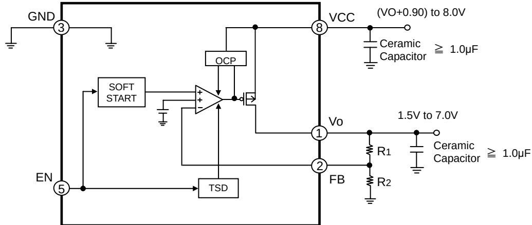
Fig.1 Block Diagram
