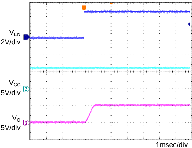
Fig.16 Input sequence 2 \text{Co}=1\mu\text{F} , T_a=25^{\circ}\text{C}
