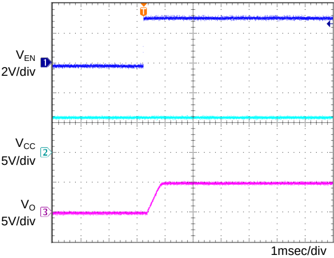
Fig.17 Input sequence 2 \text{Co}=1\mu\text{F} , T_a=105^{\circ}\text{C}
