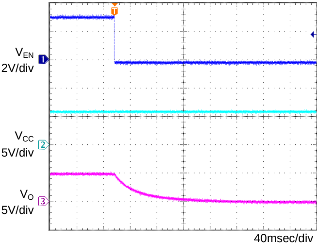
Fig.18 OFF sequence 2 \text{Co}=1\mu\text{F} , T_a=-40^{\circ}\text{C}
