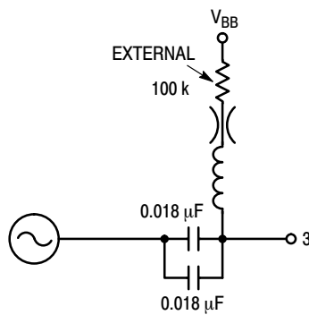
NF TEST CONDITIONS I_C = 1.0\text{ mA} V_{CE} = 6.0\text{ VOLTS} R_S = 50\ \Omega f = 60\text{ MHz}
