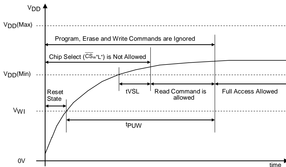
Figure 25. Power-on Timing
