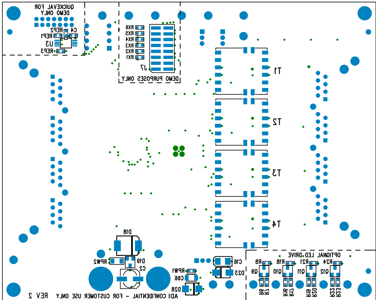
Bottom Assembly
