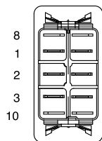
BOTTOM VIEW TERMINAL ARRANGEMENT 10 TERMINAL BASE
