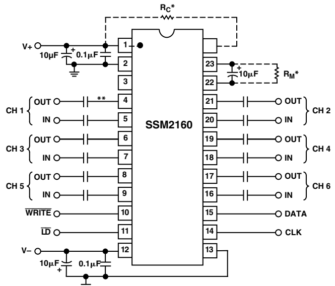
Figure 13. Typical Application Circuit (Dual Supply)
