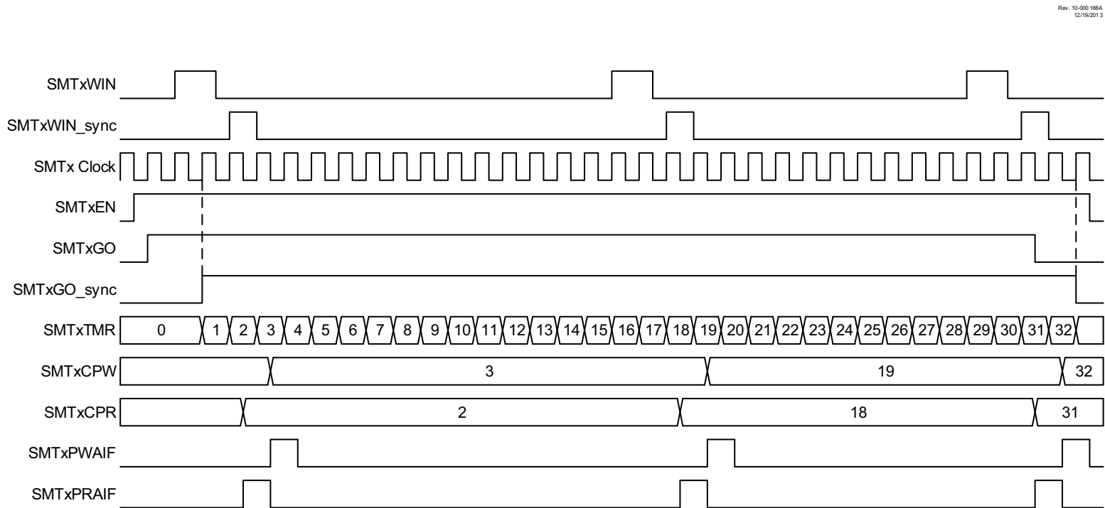
FIGURE 28-16: CAPTURE MODE REPEAT ACQUISITION TIMING DIAGRAM
