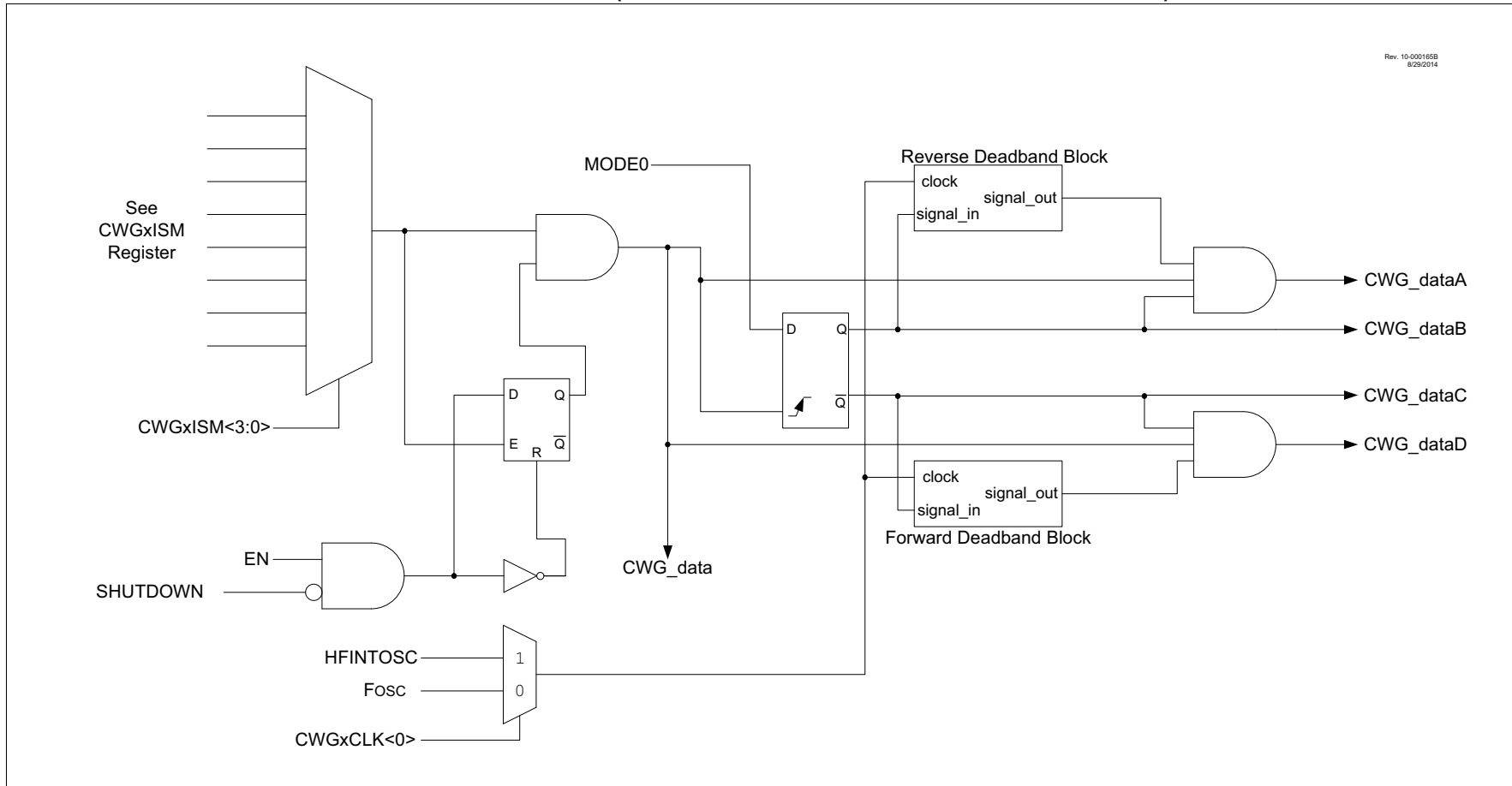
PIC16(L)F19195/6/7
