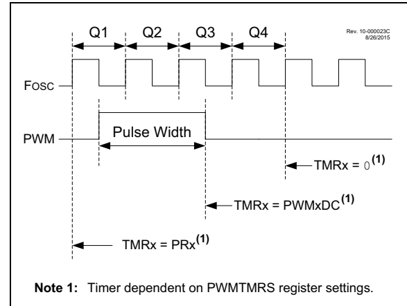
FIGURE 30-1: PWM OUTPUT
