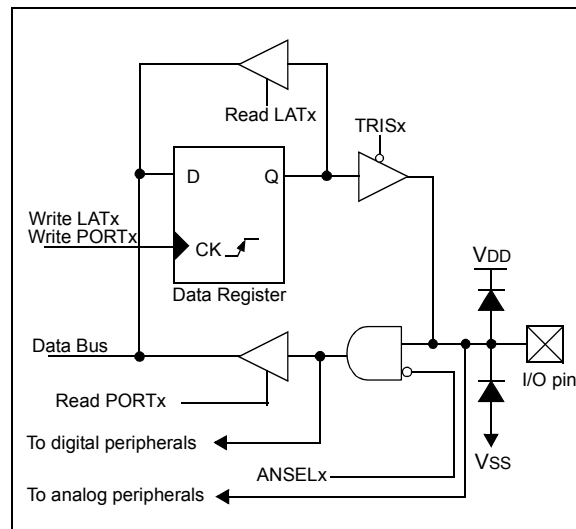
FIGURE 14-1: GENERIC I/O PORT OPERATION
