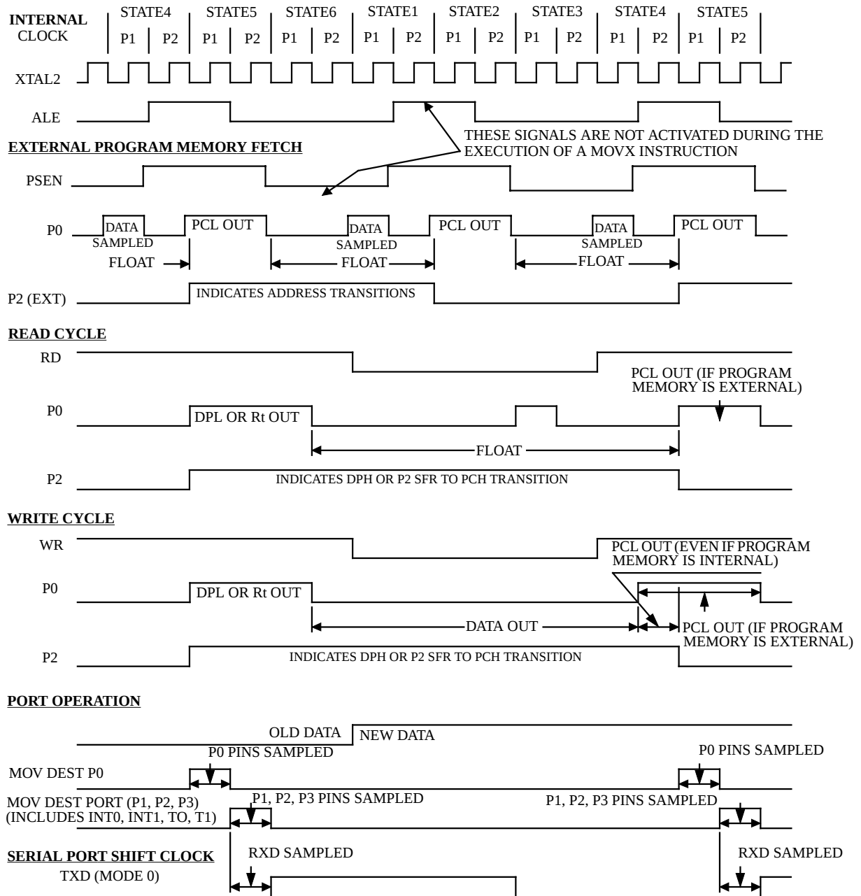
Figure 29. Clock Waveforms
