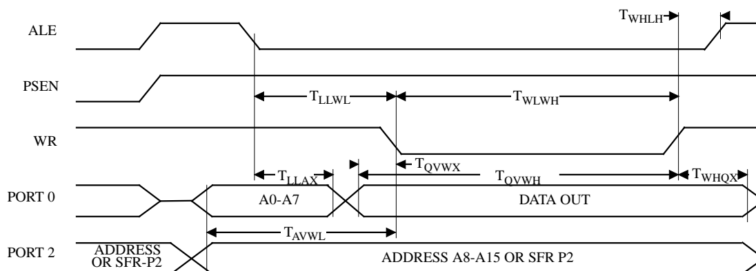
Figure 22. External Data Memory Write Cycle
