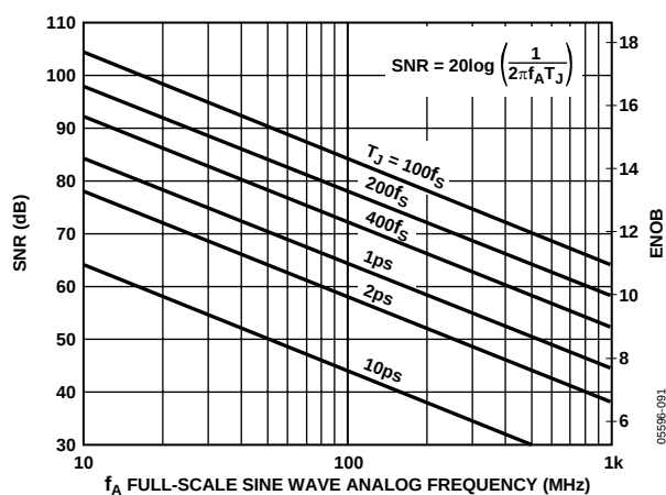
Figure 35. ENOB and SNR vs. Analog Input Frequency
