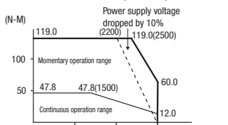
R88M-KH7K515C (7.5 kW)
