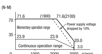
R88M-KH5K020F/C (400 V, 5 kW)
