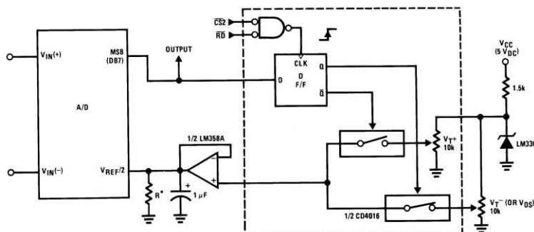
Figure 27. \mu P Compatible Differential-Input Comparator with Pre-Set VOS (with or without Hysteresis)
