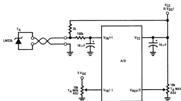
Figure 29. Low-Cost, \mu P Interfaced, Temperature-to-Digital Converter
