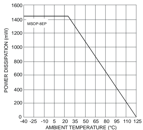
Figure 5. Derating Curve
