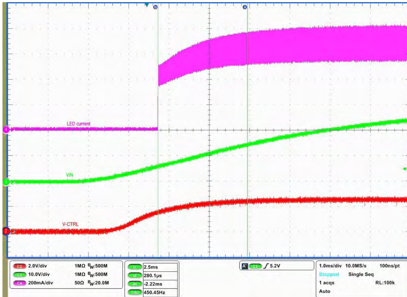
Figure 4. Soft Start with 22nF Capacitor on CTRL Pin ( V_{IN} = 36V , I_{LED} = 667mA , 1 LED)
