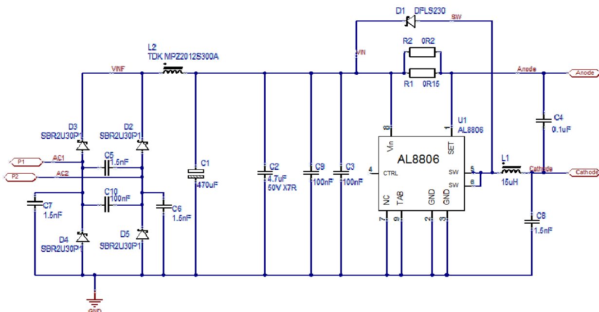
Figure 7. MR16 Schematic
