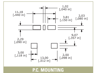
P.C. MOUNTING
